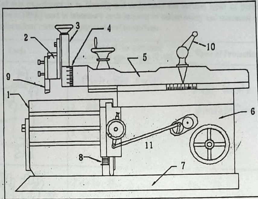
Fig: Shaper machine
